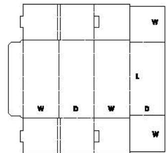
0470 Roll End Tray with Tuck Top and Interior Bottom Flaps or Reverse Walker Lock with Inside Tuck Top
