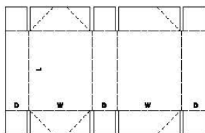
0760 Self Erecting Six Corner Tray
