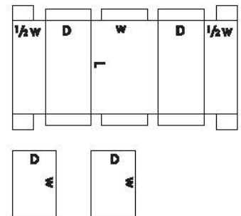
0606B Bliss Style Container with End Panel Legs
