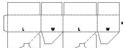
0711 Pre-glued Auto Bottom with RSC Top Flaps
