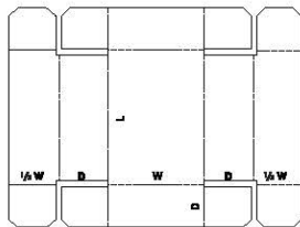
0416 One Piece Folder (OPF), Die Cut with Dust and Tuck Flaps
